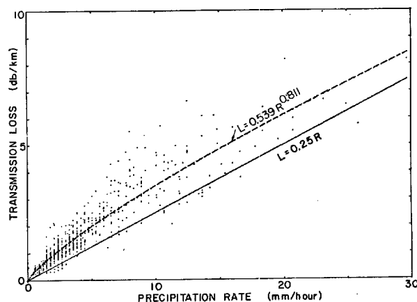
Fig. 3. Comparison of experimental and theoretical rain attenuation data.
