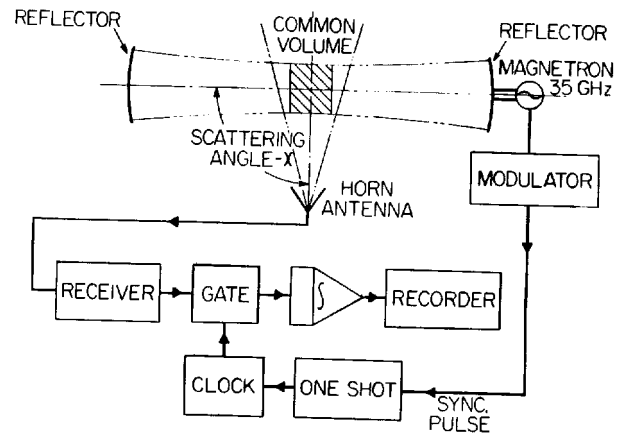
Fig. 4. Rain side-scatter measuring system.
