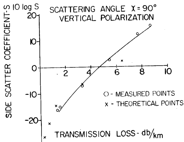
Fig. 5. Measured data for rain side scatter.
